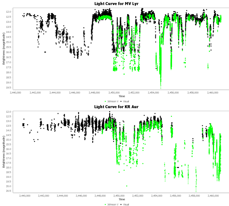
Fig. 1. Long-term light curves of MV Lyr (1970–2025, top) and KR Aur (1967–2005, bottom) from AAVSO.
