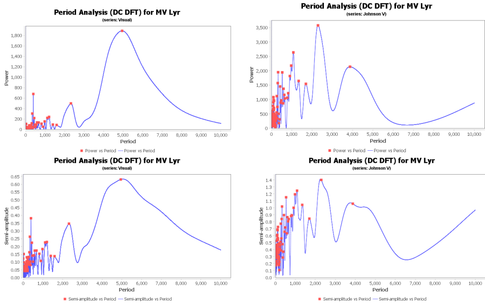
Fig. 2. Periods and their semi-amplitudes in visual and Jonson’s V observations of MV Lyr.
