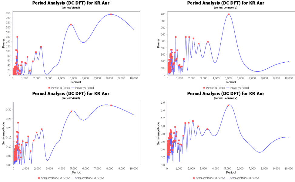
Fig. 3. Periods and their semi-amplitudes in visual and Jonson's V observations of KR Aur.
