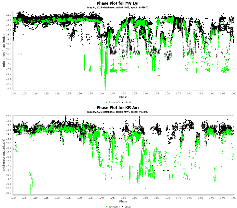
Fig. 4. Phase curves with the best periods for MV Lyr (top) and KR Aur (bottom).
