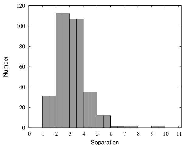
Fig. 3. Distribution of the angular separations of the measurements. The unit for separation is arcsecond.
