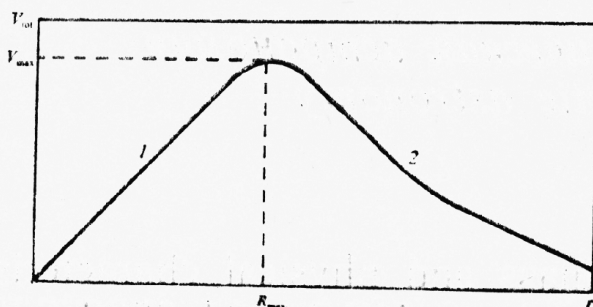
Fig. 1. General view of the rotation curve of a spiral galaxy. Distance r from the centre of the galaxy is plotted along the abscissa, and rotation velocity V_{rot} in km/s is plotted along the ordinate.
