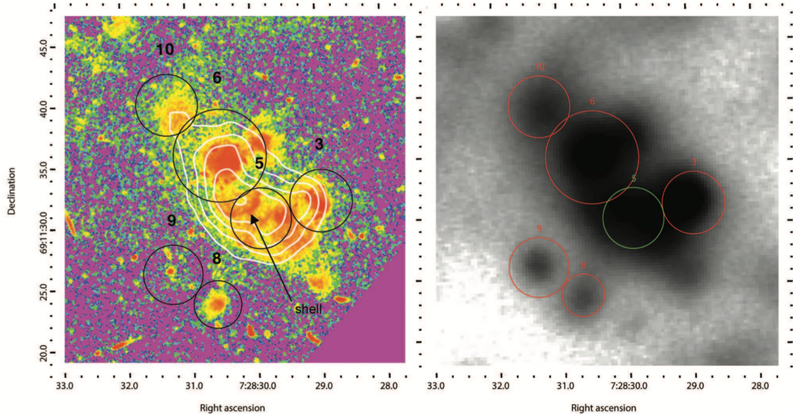
Fig. 6. Left: HST WFPC2 F658N image with overlaid [SII] contours, centered on the starforming region near the object Vu19 5. The maximum of [SII] emission aligns with the partial H \alpha shell resolved with HST. Right: the same part of our H \alpha image. Seeing was 3''.25. The diameter of the SNR candidate Vu19 5 is 5''.0=85 pc.
