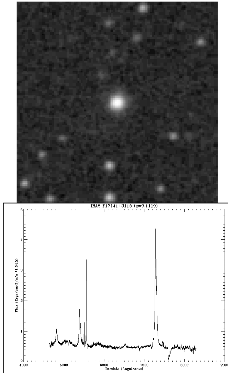
Fig. 1. Upper panel: a 2 \times 2 arcmin wide POSS-II red image of IRAS F17141+3115; North is at the top, East is to the left. Lower panel: a spectrum of the object taken at OHP.
