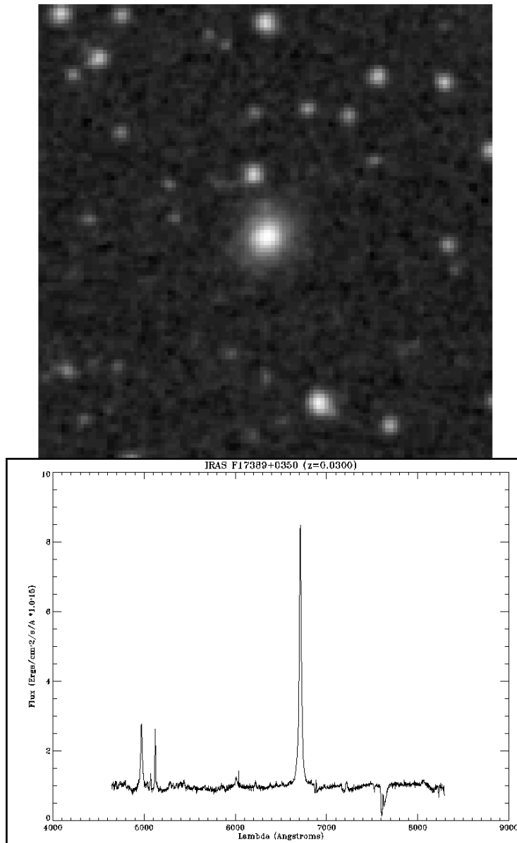
Fig. 2. The same as in Fig. 1, but for IRAS F17389+0350.
