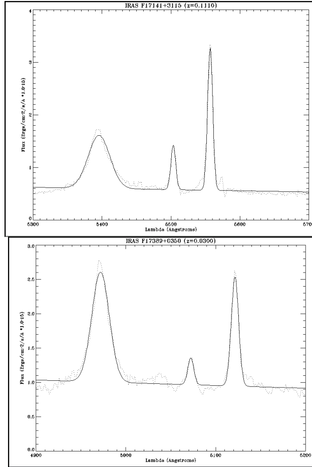
Fig. 3. A decomposition of the H\beta + [OIII] spectral region (dots) using unweighted 3-component Gaussian fit (solid line) for IRAS F17141+3115 (upper panel) and for IRAS F17389+0350 (lower panel).
